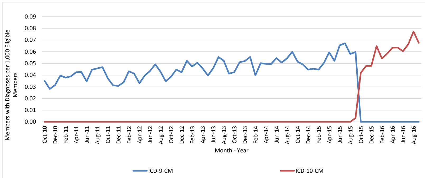
Figure 2. Prevalence of Rhabdomyolysis Diagnoses per 1,000 Eligible Members from October 2010 - August 2016, by Code Type, 0-Day Washout
