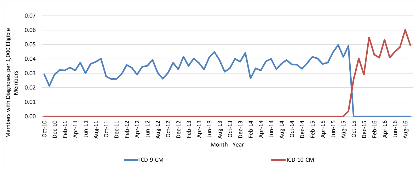
Figure 1. Incidence of Rhabdomyolysis Diagnoses per 1,000 Eligible Members from October 2010 - August 2016, by Code Type, 183-Day Washout
